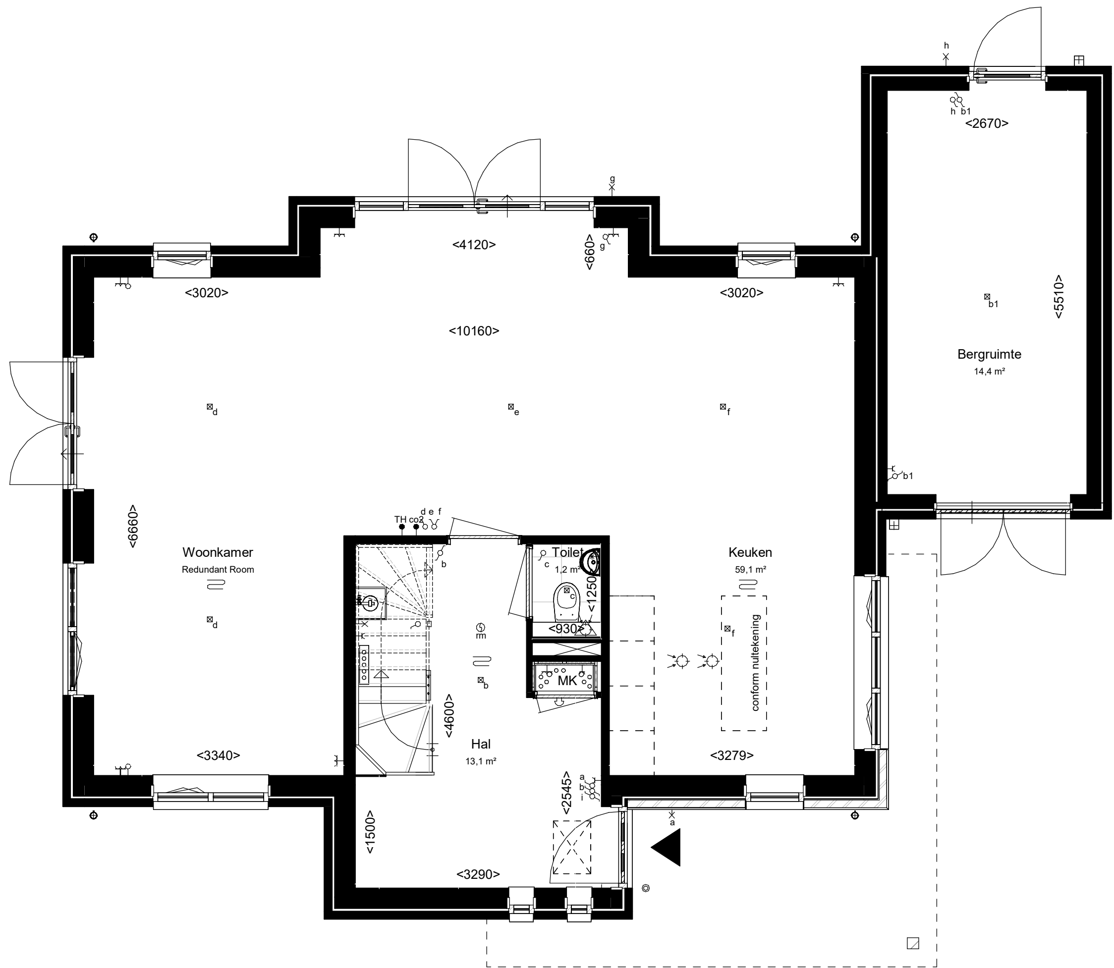
Begane grond, PEIL=0
